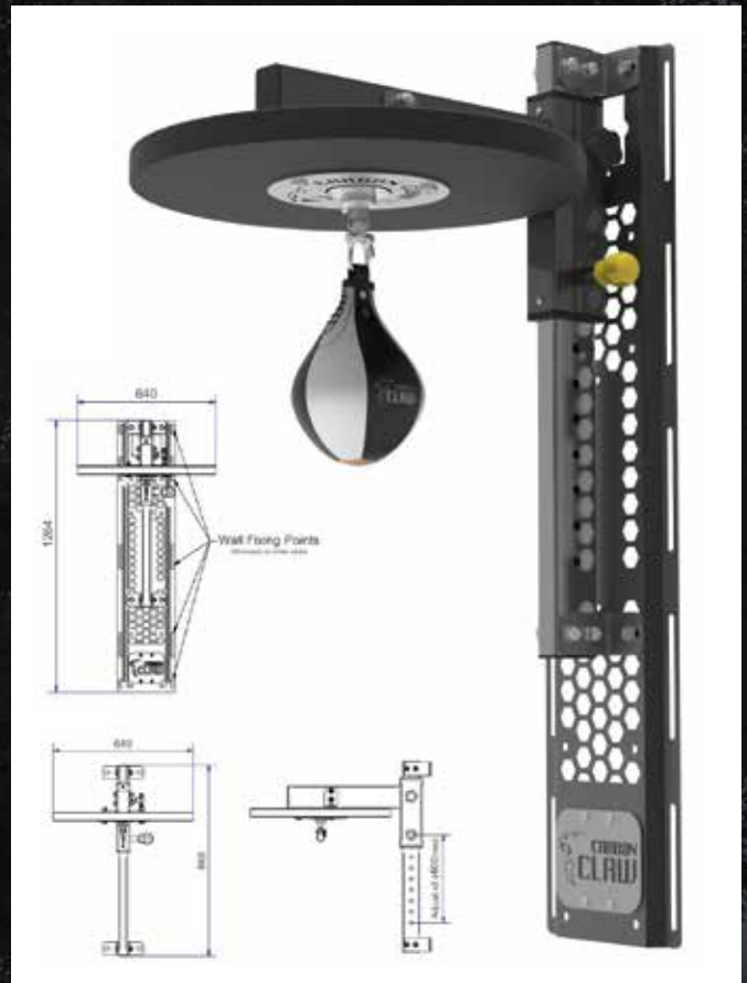
LASER CLUB PRO SPEEDBALL FRAME CC-577
